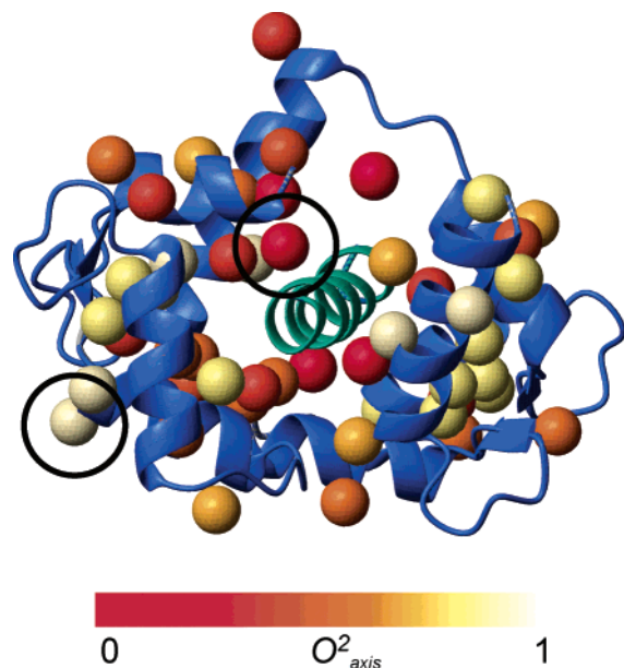
Figure 4. Distribution of amplitude of fast motion of methyl groups in a calmodulin/peptide complex. Shown is a ribbon representation of the backbone of the crystal structure (1CDL) 141 of the complex between calcium-saturated calmodulin and a peptide representing the calmodulin binding domain of the smooth muscle myosin light chain kinase. Methyl groups are represented by spheres that are color-coded according to their O^2_{axis} parameter determined by deuterium relaxation. 106 Note the circled methyl groups illustrating that being on the surface of the protein does not necessarily result in extensive amplitude of motion nor does complete burial necessarily result in highly restricted motion.
