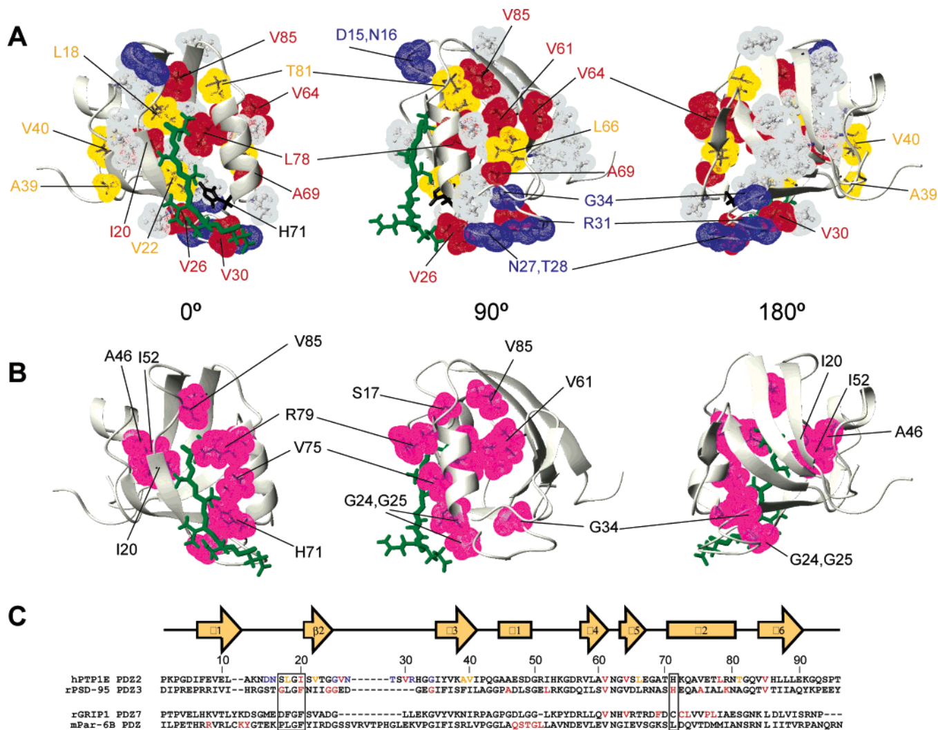
Figure 14. Comparison between dynamically linked residues in a PDZ domain and thermodynamic couplings predicted from a family of PDZ domains. (A) A summary of residues whose dynamical parameters change significantly upon peptide binding mapped onto the structure of the PDZ2/RA-GEF2 complex. The PDZ2 protein secondary structure is colored gray while the peptide ligand is green. Red VDW surfaces are side chain methyl residues that had appreciable \Delta O_{\text{axis}}^2 , in yellow are those methyl residues with appreciable \Delta \tau_e , and in blue are backbone NH groups that displayed changes in motion on the chemical shift time scale. Methyl groups not having changes in dynamics parameters are represented as gray VDW surfaces. Residues that were not compared are shown in black. For clarity, three views are presented. Residues of importance are labeled. (B) The statistical couplings derived from Lockless and Ranganathan 119 are mapped onto the PDZ1/RA-DEF2 structure shown in identical views as in part A. (C) Primary sequences of four PDZ domains color coded as in part A. See Fuentes et al. 122 for more detail. Reprinted from Journal of Molecular Biology 335, Fuentes, E. J., Der, C. J., Lee, A. L., Ligand-dependent dynamics and intramolecular signaling in a PDZ domain, pages 1105–15, Copyright 2004, with permission from Elsevier.
