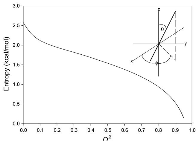
Figure 15. Parametric relationship between the generalized order parameter, reported by a nuclear interaction vector situated as a spy on an azimuthally symmetric harmonic oscillator, and the corresponding entropy. 92 Here a simple quadratic potential is used and a parametric relationship exists between the entropy of the oscillator (inset) and the O^2 parameter created by varying the force constant governing the potential energy. Uncertainty in the reduced mass, the depth of the energy well, and the effective length of the oscillator reduces the utility of the method for obtaining absolute entropies. However, estimates of differences in entropy are anticipated to be at least semiquantitative (see text).
