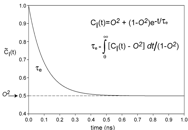
Figure 1. Schematic illustration of the Lipari–Szabo model-free internal autocorrelation function describing the motion of a nuclear spin interaction vector within the molecular frame of an isotropically tumbling macromolecule. 60 The square of the generalized order parameter ( O^2 ) defines the contribution of internal motion to the decay of the autocorrelation function. The effective correlation time ( \tau_e ) is defined as the normalized area under the internal correlation function. This particular example was simulated with O^2 of 0.5, \tau_e of 200 ps, and an isotropic global reorientation correlation time ( \tau_m ) of 10 ns. Note, the original Lipari–Szabo treatment utilizes the symbol S to denote the generalized order parameter. To avoid confusion with the similar symbol corresponding to entropy, we shall employ O throughout to denote the generalized order parameter.
