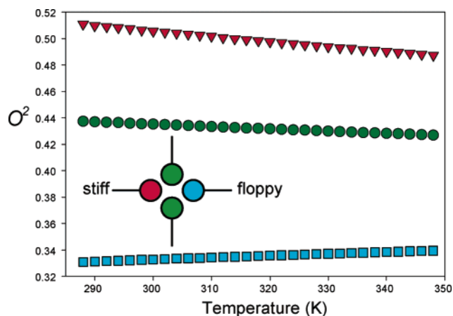
Figure 10. Temperature dependence of O^2 parameters of sites attached to four interacting side chains in a two-dimensional cluster model (inset). The green side chains have the same temperature dependence (●), the stiff red side chain (▼) and floppy blue side chain (■) have negative and positive temperature dependencies, respectively. Adapted with permission from ref 93. Copyright 2002 American Chemical Society.
