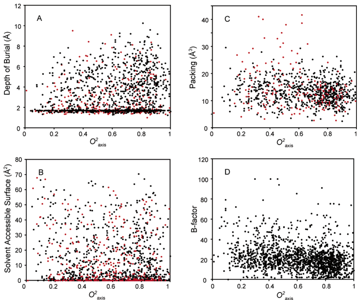
Figure 3. Correlation of experimentally determined methyl group dynamics with several primitive structural parameters. Methyl group symmetry axis squared generalized order parameters ( O_{\text{axis}}^2 ) determined by deuterium relaxation were obtained from the literature (Table 2). Structural parameters were obtained from structural models determined by crystallography (black symbols) or by NMR spectroscopy (red symbols). Panel A: Correlation of O_{\text{axis}}^2 with depth of burial. Depth of burial was calculated by determination of the shortest distance between the methyl carbon and a molecular surface created with a rolling sphere (1.4 Å radius) utilizing the GRASP program. 140 Panel B: Correlation of O_{\text{axis}}^2 with solvent accessible surface area. The solvent accessible surface area was determined using a rolling sphere with a radius of 1.4 Å. Panel C: Correlation of O_{\text{axis}}^2 with packing density as determined by subtraction of the van der Waals volume of the methyl group from the volume of the Voronoi polyhedral. Packing density was determined only for buried sites (i.e. atoms with completed Voronoi polyhedra). Panel D: Correlation of O_{\text{axis}}^2 with crystallographic B -factors. In no case does the R^2 of the best fitted line to any of these data sets exceed 0.05.
