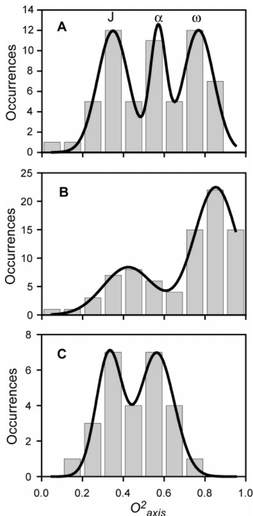
Figure 5. Histograms of the distribution of squared generalized order parameters of methyl group symmetry axes ( O^2_{axis} ) in (A) the complex of calcium-saturated calmodulin and a peptide derived from the calmodulin binding domain of the smooth muscle myosin light chain kinase, 106 (B) flavodoxin, 100 and (C) \alpha_3d , a protein of de novo design. 101 Lines are best fits to a sum of three Gaussians for part A, giving R^2 = 0.989 , and to a sum of two Gaussians for parts B and C, giving R^2 = 0.999 and 0.986 , respectively.
